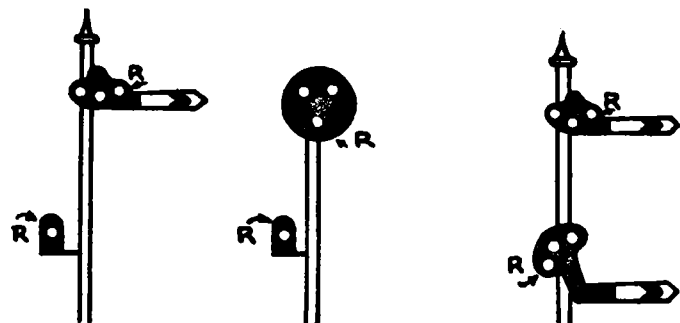
Indication—Stop—Then proceed in accordance with Rule 509 or 660. Name—Stop and Proceed Signal.
