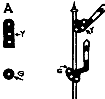
Indication—Train approach next signal at not exceeding one-half its maximum authorized speed at point involved but not exceeding 30 miles per hour.
