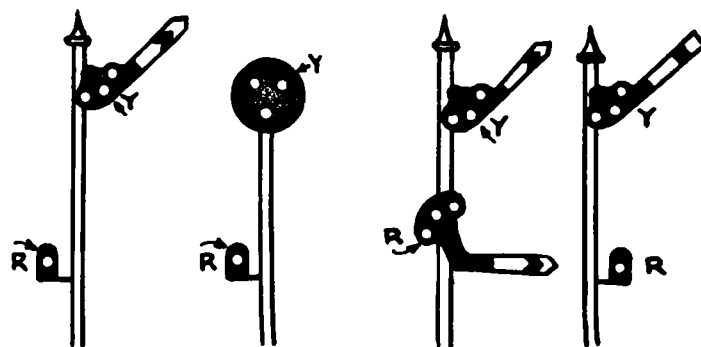
Indication—Approach next signal prepared to stop. A train exceeding one-half its maximum authorized speed at point involved must at once reduce to not exceeding that speed.
