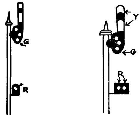
Indication—Proceed manual or controlled manual block clear. Name—Clear Block Signal.
